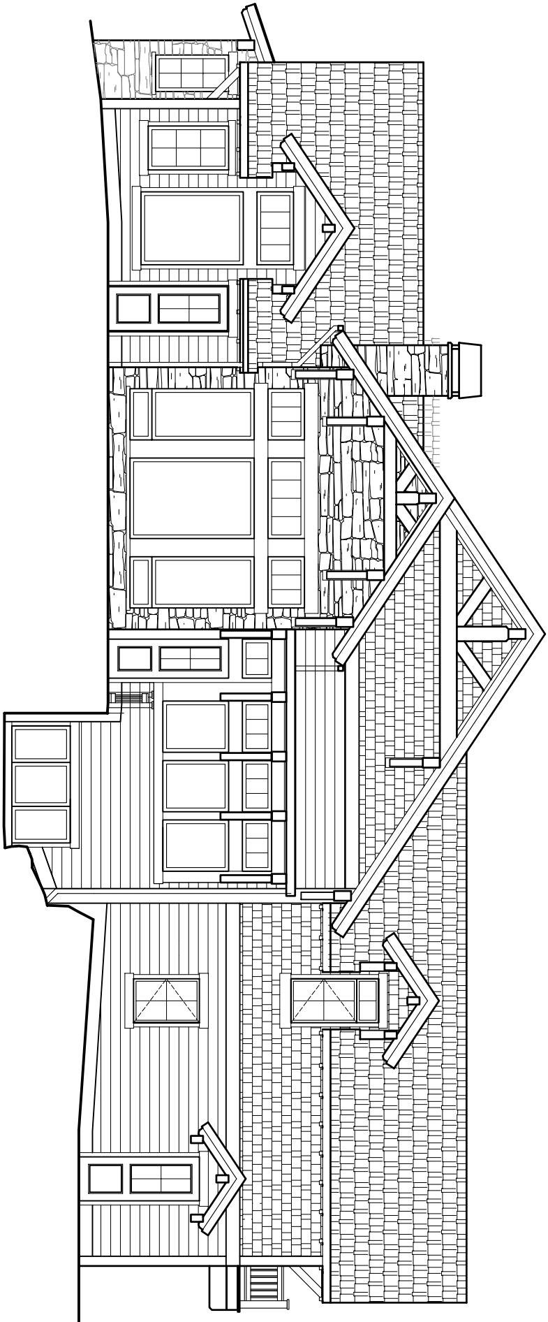
EAST EXTERIOR ELEVATION
