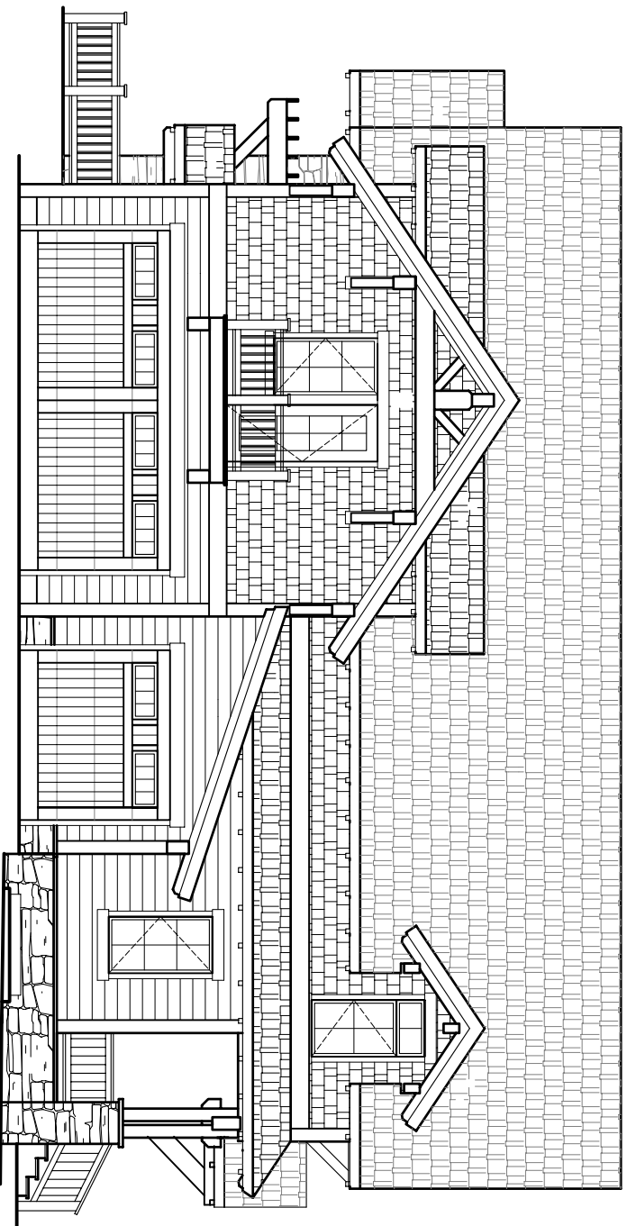
NORTH EXTERIOR ELEVATION
