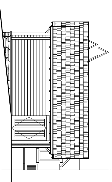
GARAGE SOUTH EXTERIOR ELEVATION
